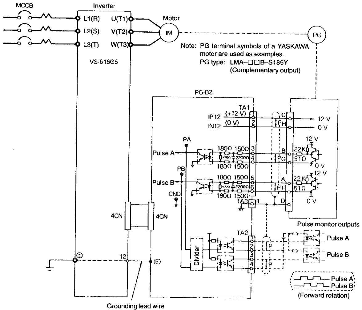
Fig. 4 Interconnection diagram
