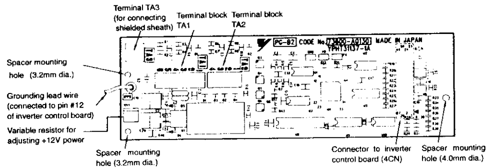
Fig. 1 PG speed controller card PG-B2
